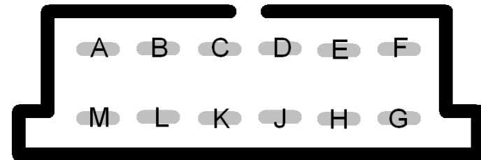
ALDL 12-pin Plug
